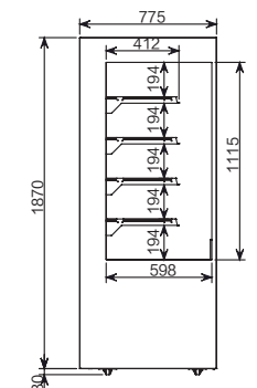
侧视图 Side View
