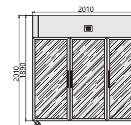
JF1800C
