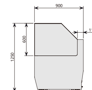
侧视图 Side View
