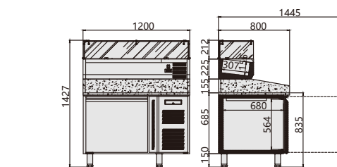
PZ1100TN/380
