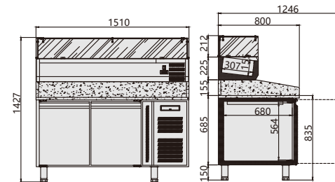
PZ2600TN/380
