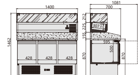
PZ903/380
