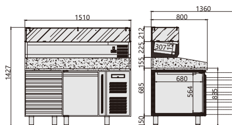
PZ1610TN/380
