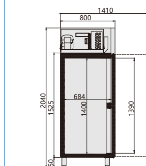
侧视图 Side View
