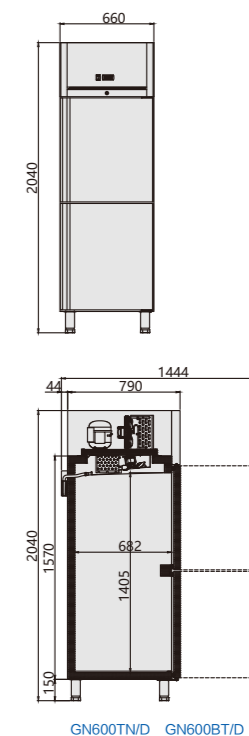
GN600TN/D GN600BT/D
